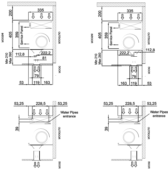
Standard Installation
